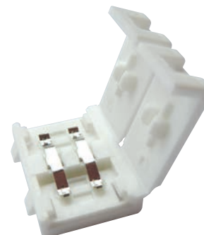
LED 8mm Tape Butt Connector K30-5815
